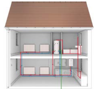
Unvented system
